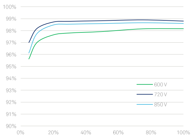
Efficiency Curve SUN2000-60KTL-M0 @480 V
