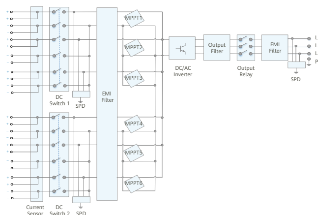
Circuit Diagram
